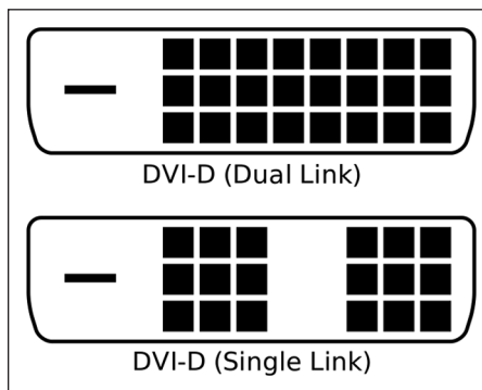
FIGURE 1-14: Two different kinds of DVI-D cables — they work well, but don't carry audio.
